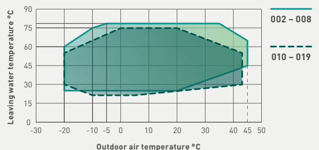
Operating map in heating mode
